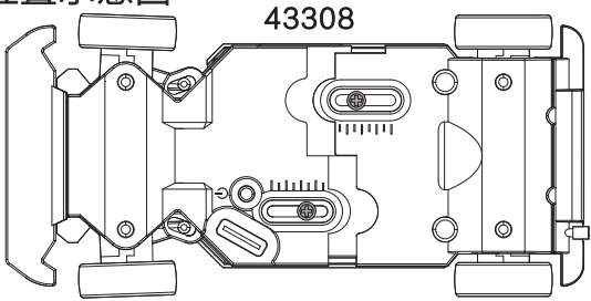
Diagram of undercarriage bolt installation locations 车底螺丝安装位置示意图
