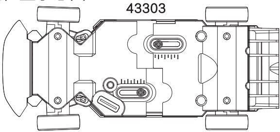
Diagram of undercarriage bolt installation locations 车底螺丝安装位置示意图
